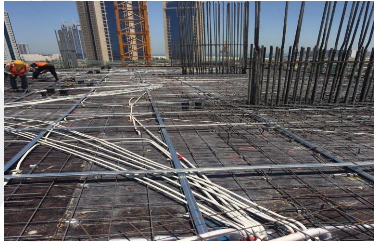
9 th Floor – Steel Works
