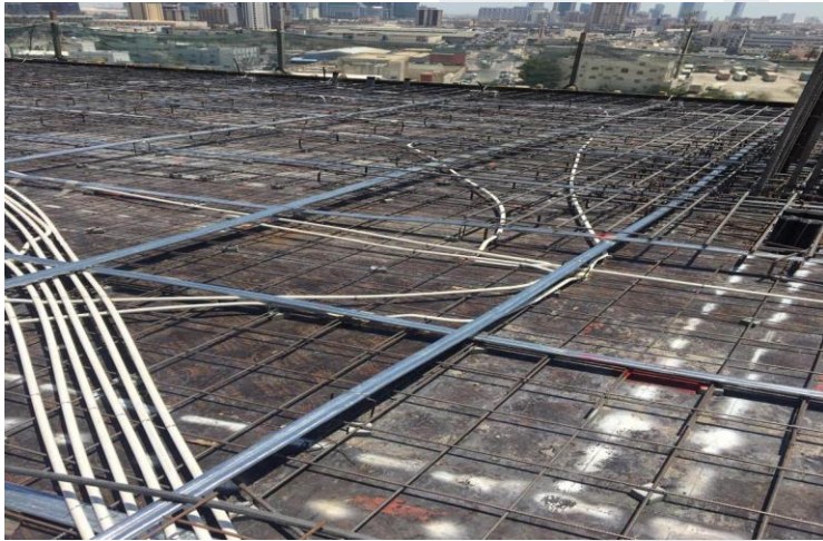
9 th Floor – Steel Works
