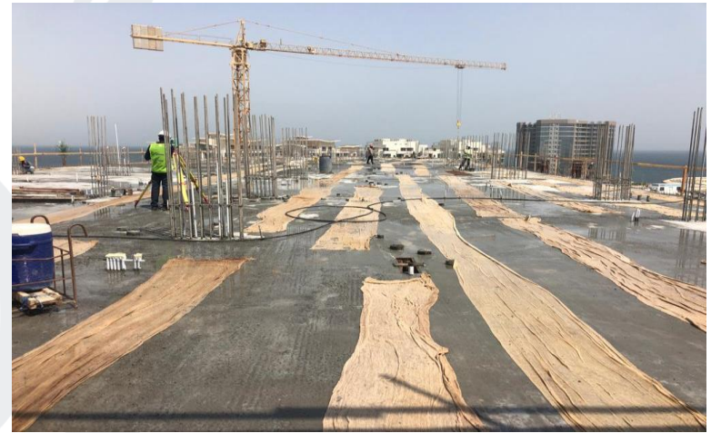
Zone 2 – 6 th Floor Slab & Beam Shuttering and reinforcement, Slab Concrete Works
