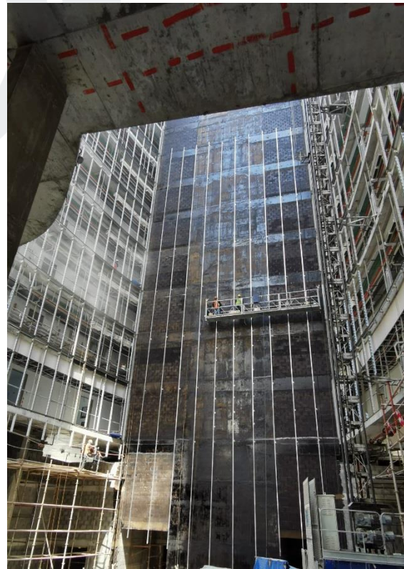
Installation of Aluminum Works (Brackets, Mullion, Rockwool ACP Cladding & Glass and Application of Bitumen Paint)
