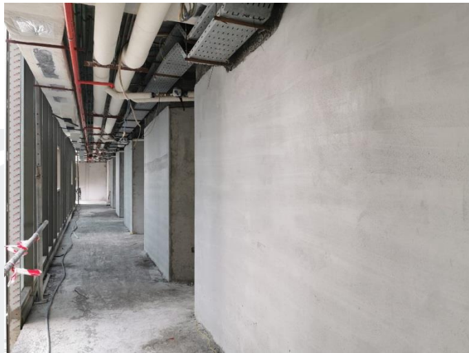
Plastering Works for Corridor Area at Typical Floors
