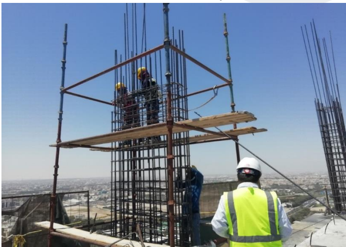
34 th Floor – Steel Work for Column
