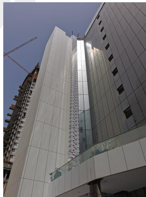
Installation of Aluminum Wall Cladding and Glass Works (External Area)
