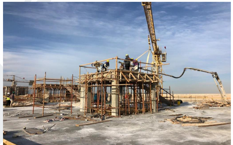
Zone 1 & 2 – Upper Roof Slab and Beam Concrete Work
